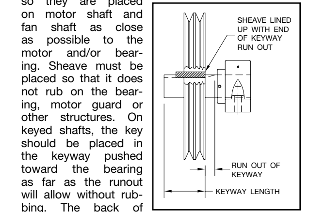
Figure 5. Sheave Position
